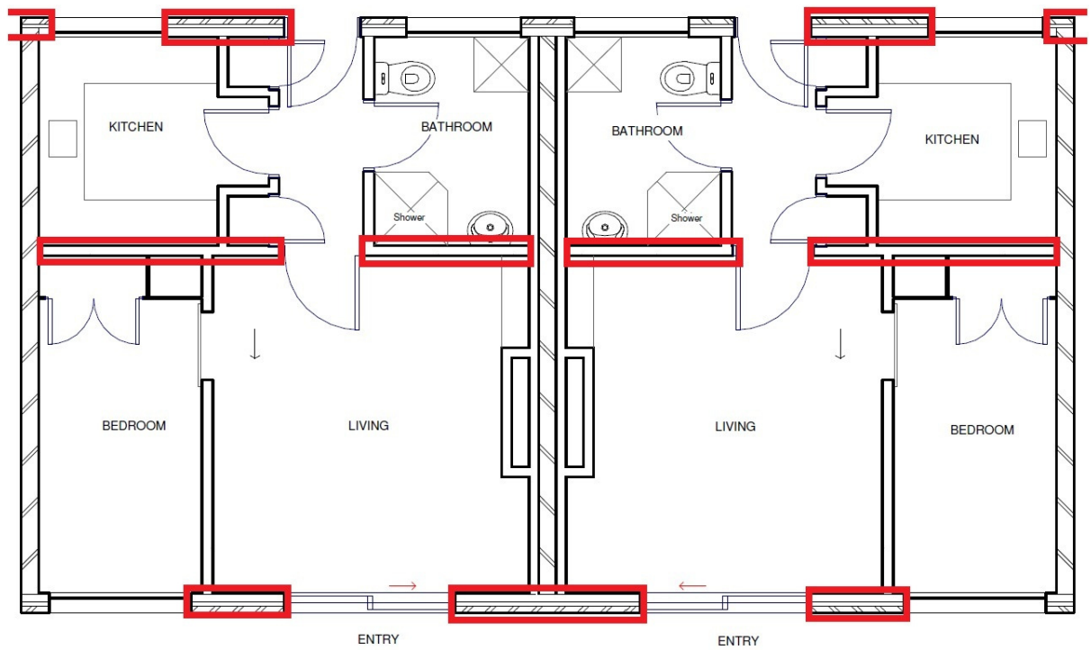
Figure 6: Walls used for bracing in the longitudinal direction
