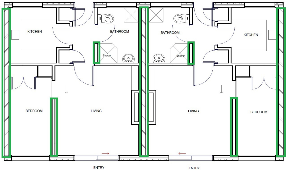
Figure 7: Walls used for bracing in the transverse direction
