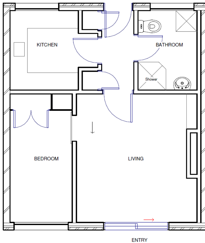
Figure 5: Partial floor plan of residential unit blocks.
