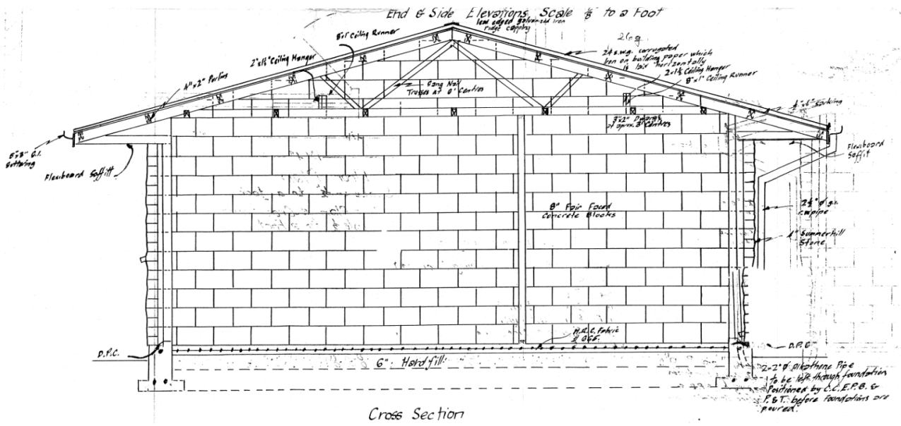
Figure 4: Typical cross section of a residential unit.
