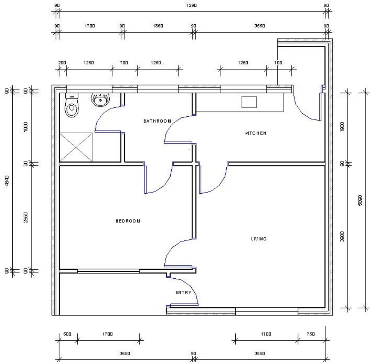
Figure 5: Typical partial floor plan of double residential units.
