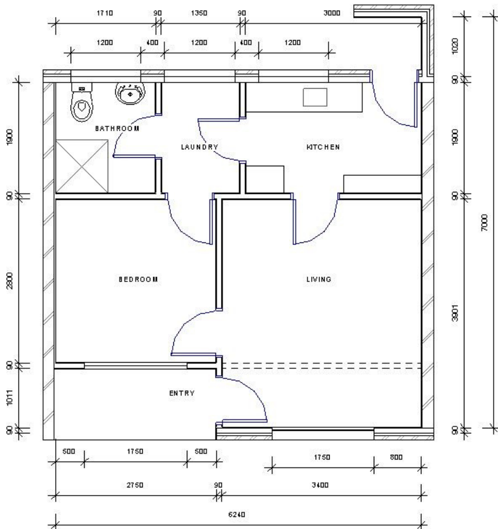
Figure 4: Typical partial floor plan of single residential units.
