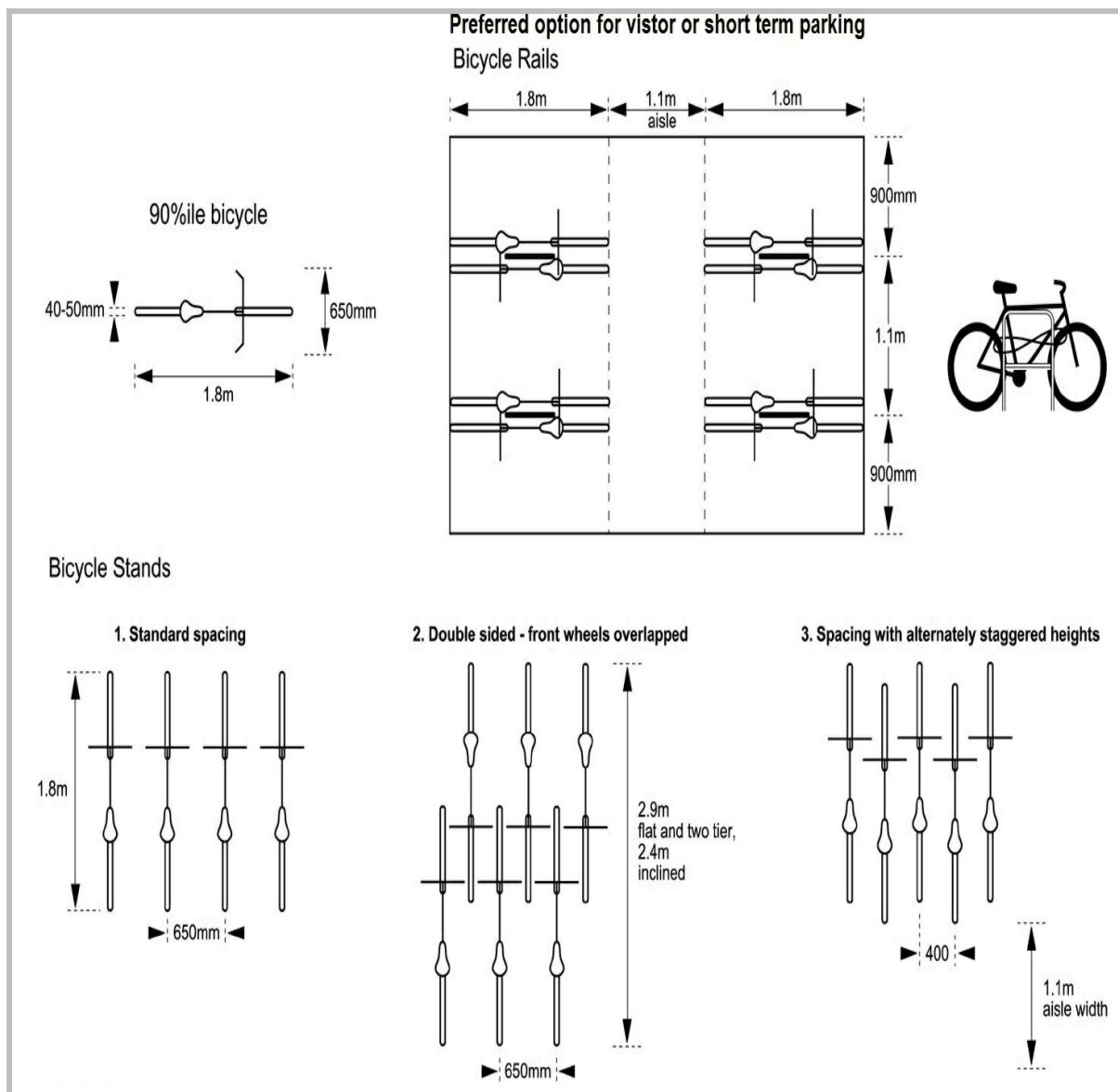
Figure 2 – Minimum cycle parking dimensions
