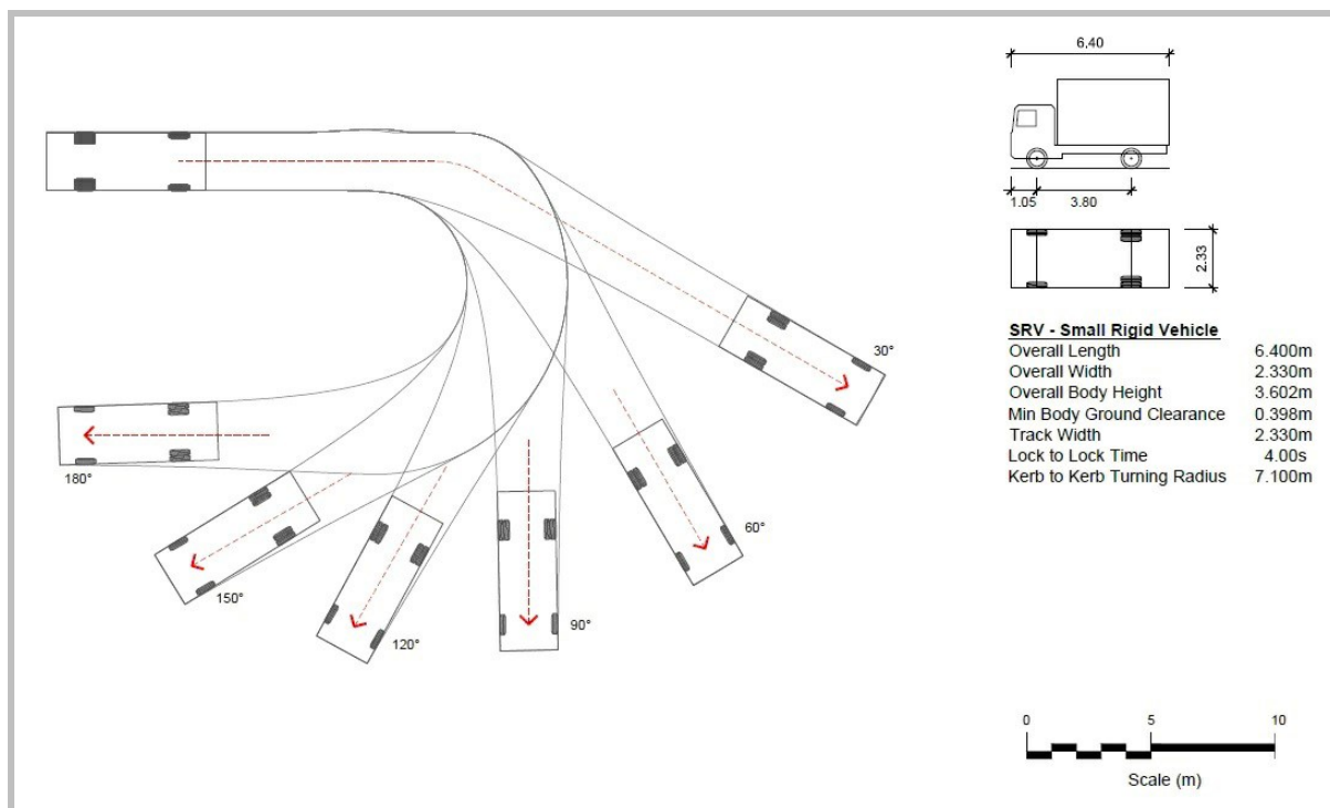
Figure 4 - Turning area for Small Rigid Vehicles
