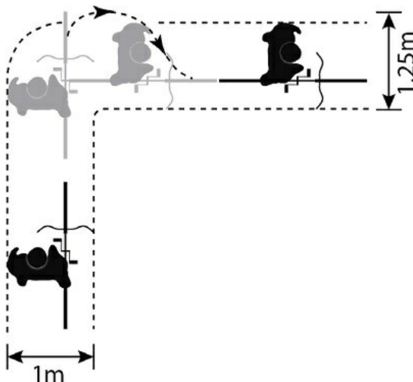
Figure 3 - Cycle turning circle - within the Central City
