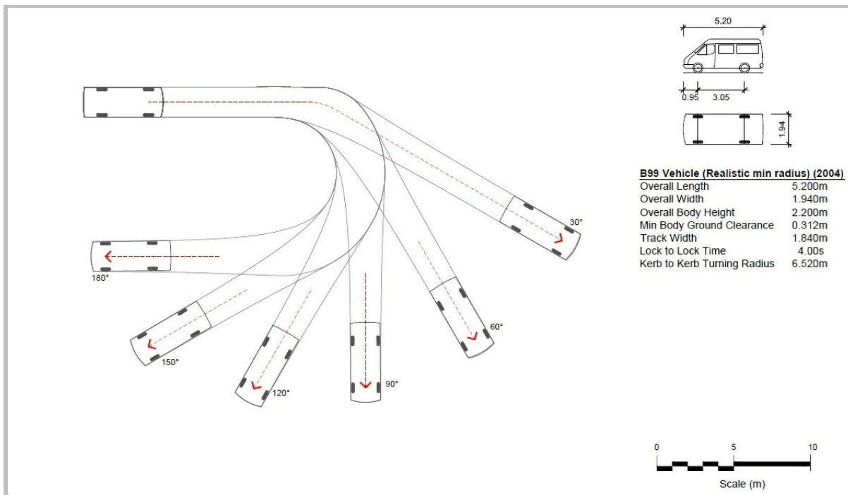
Figure 7 - 99 percentile design vehicle
