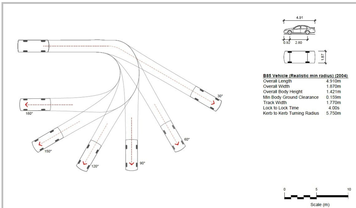
Figure 6 - 85 percentile design motor car
