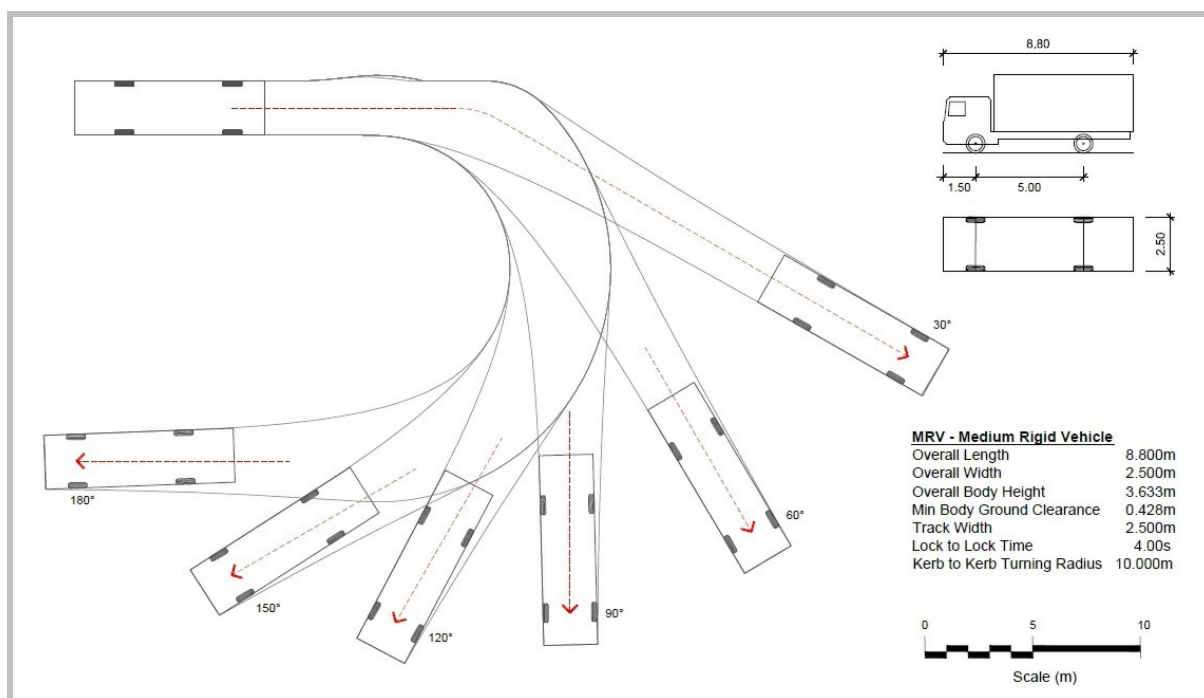
Figure 5 - Turning area for Medium Rigid Vehicles
