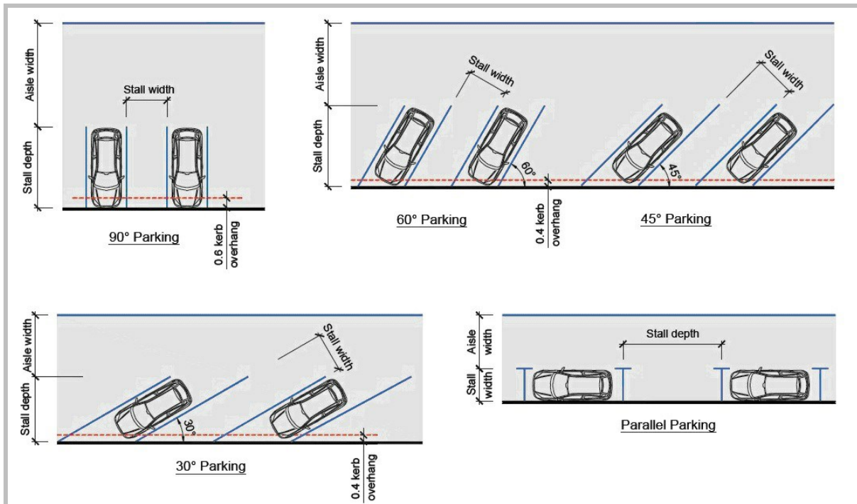
Figure 1: Car park dimensions
