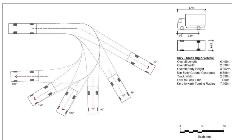
Figure 4 – Turning area for Small Rigid Vehicles
