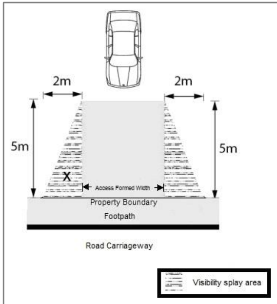
Figure 11 – Visibility splay measurement
