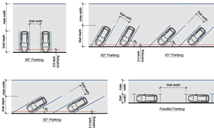
Figure 1: Car park dimensions
