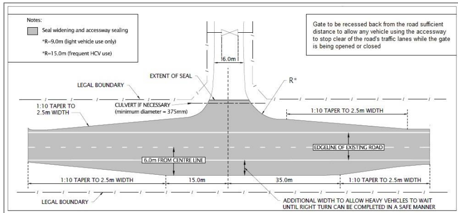
Figure 13 - Design of special use rural vehicle crossings
