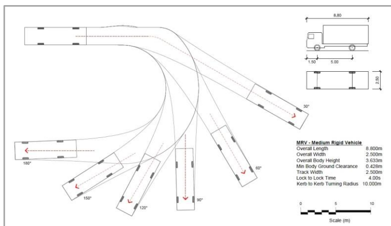
Figure 5 – Turning area for Medium Rigid Vehicles
