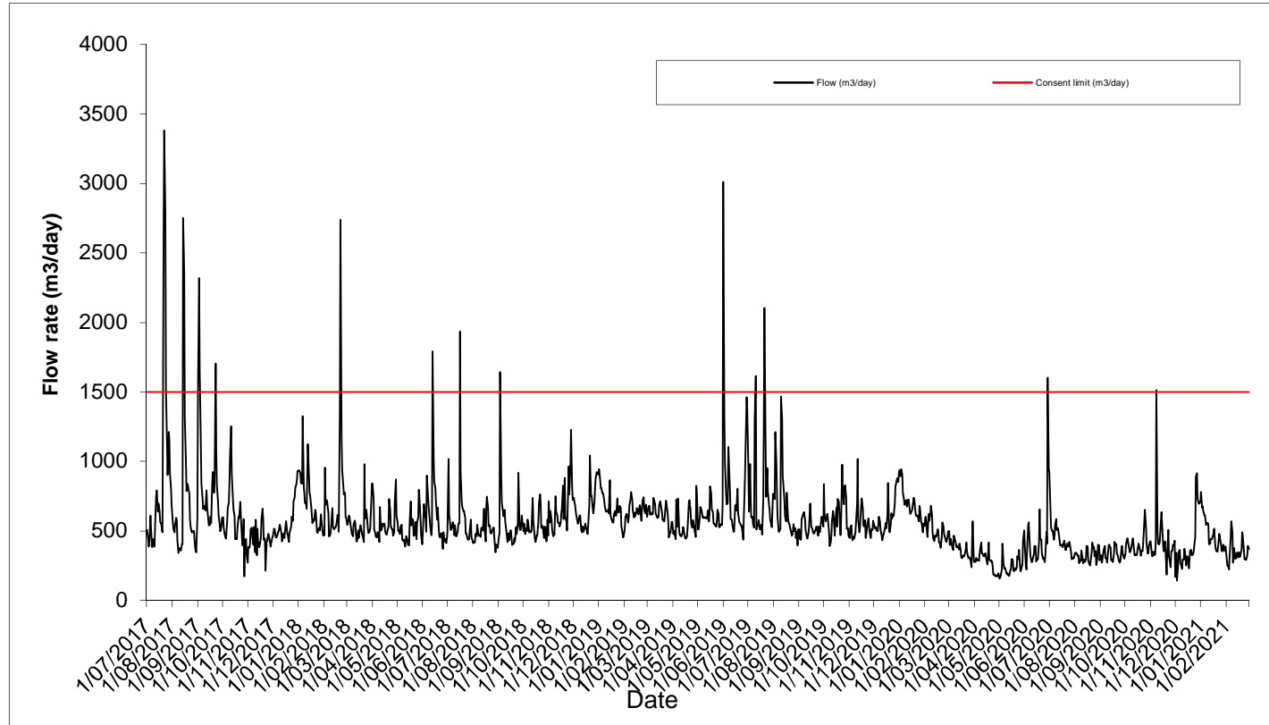
Figure 1: The daily quantity of treated water from 2017 to present at Akaroa wastewater treatment plant. cubic metres
