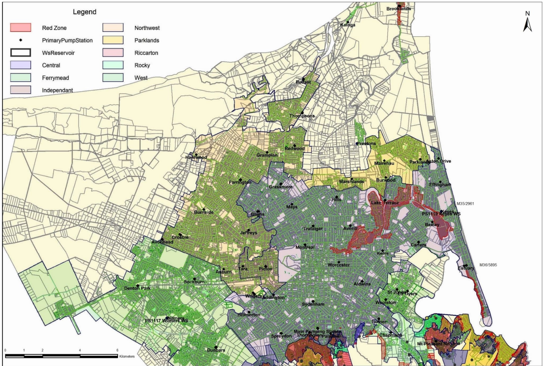
PATTLE DELAMORE PARTNERS LTD Figure 4 CCC water supply pumping station locations
