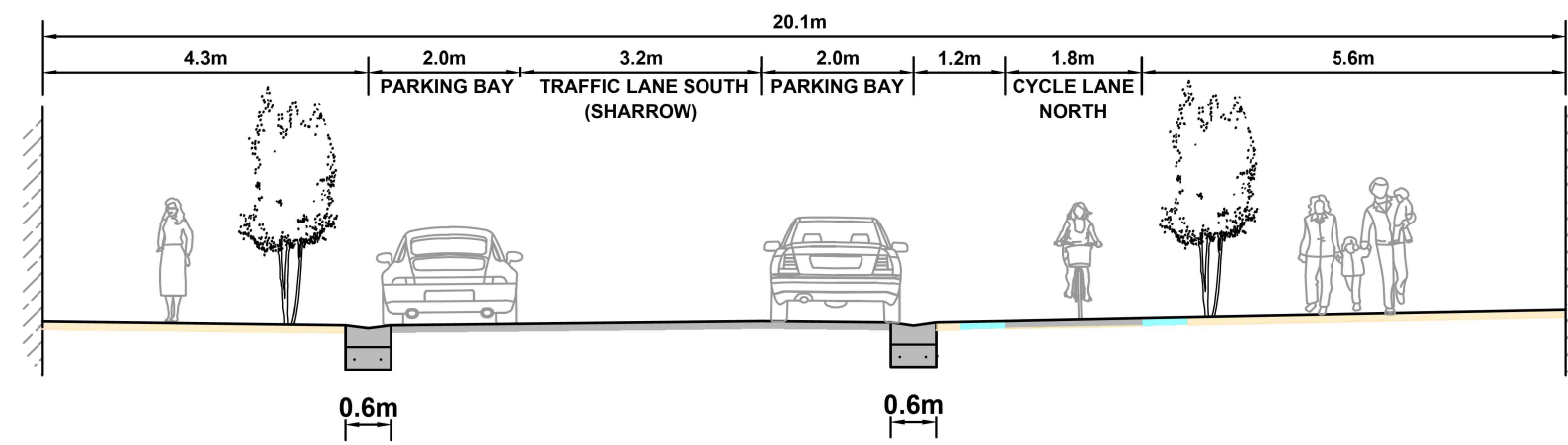
A TYPICAL CROSS SECTION SCALE 1:100
