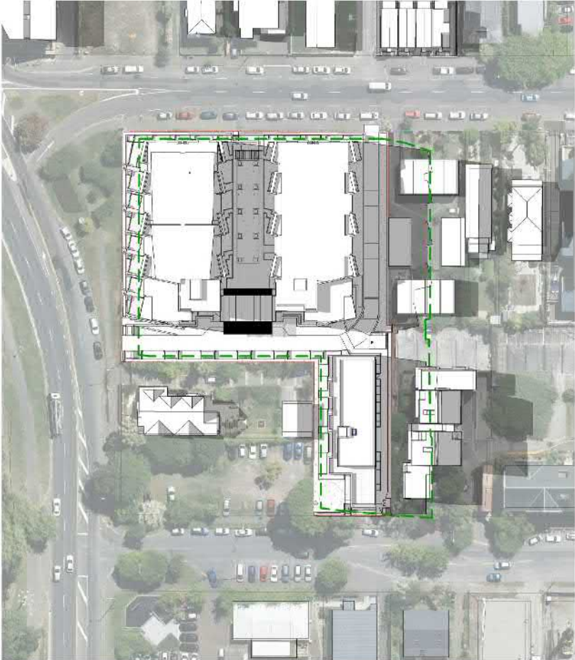
1 22 DEC 5PM CUMULATIVE A3
