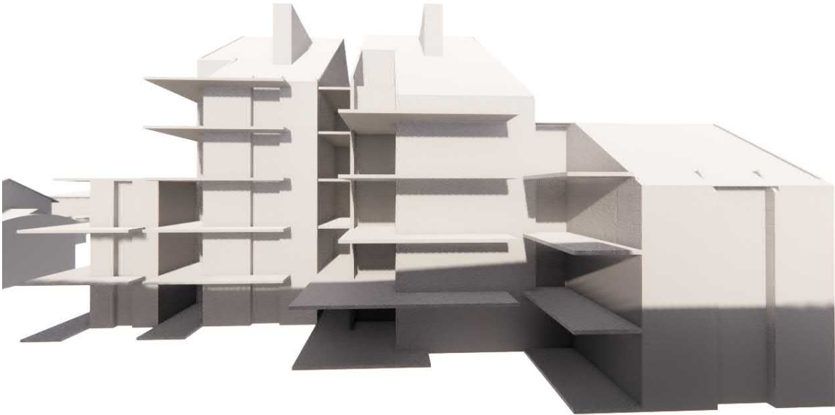
15 PETERBOROUGH ST WEST ELEVATION
