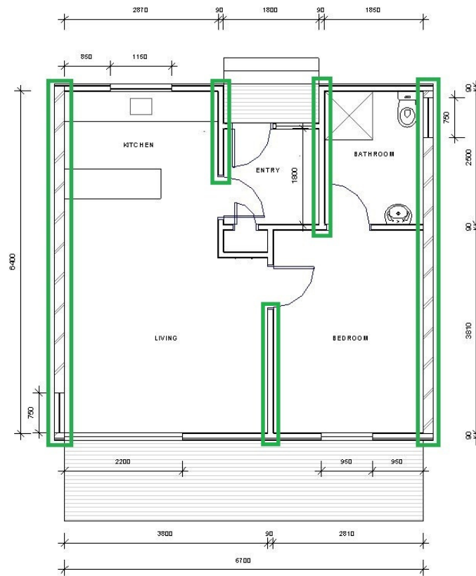
Figure 6: Walls used for bracing in the transverse direction.
