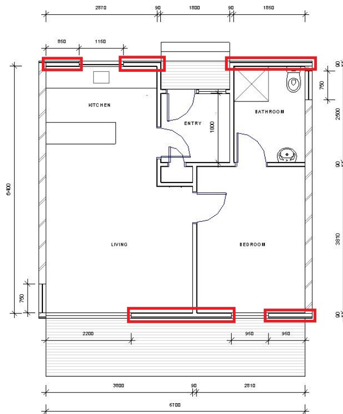
Figure 5: Walls used for bracing in the longitudinal direction.
