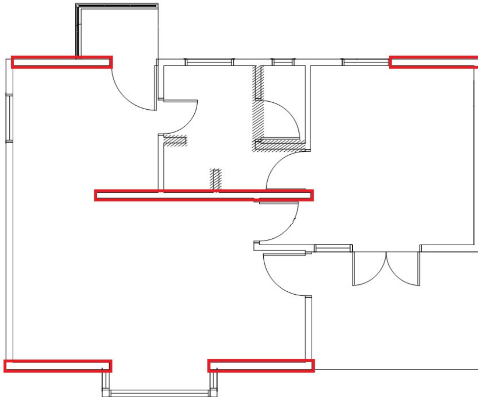
Figure 7: Walls used for bracing in the longitudinal direction.
