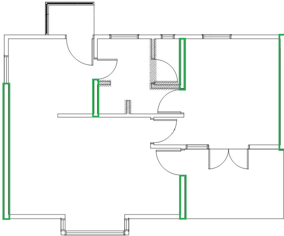
Figure 8: Walls used for bracing in the transverse direction.
