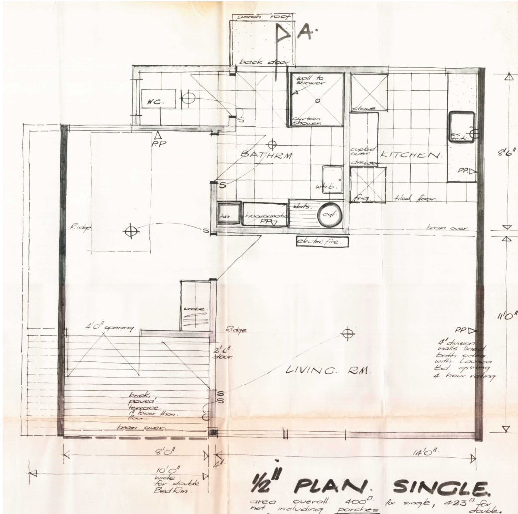
Figure 5: Typical partial floor plan of residential unit blocks.
