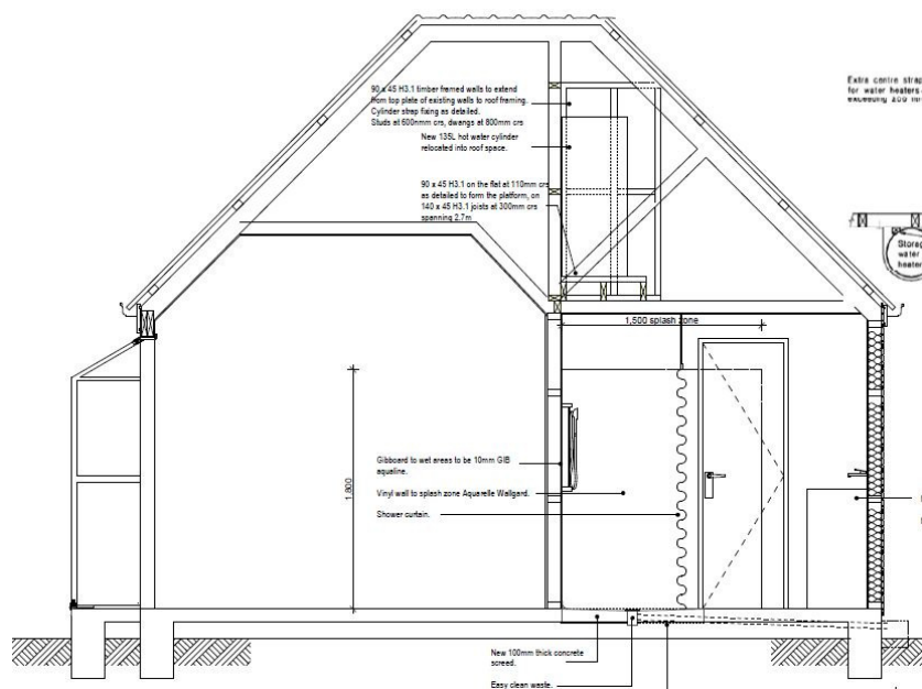
Figure 6: Cross section of Rue Viard Cottages
