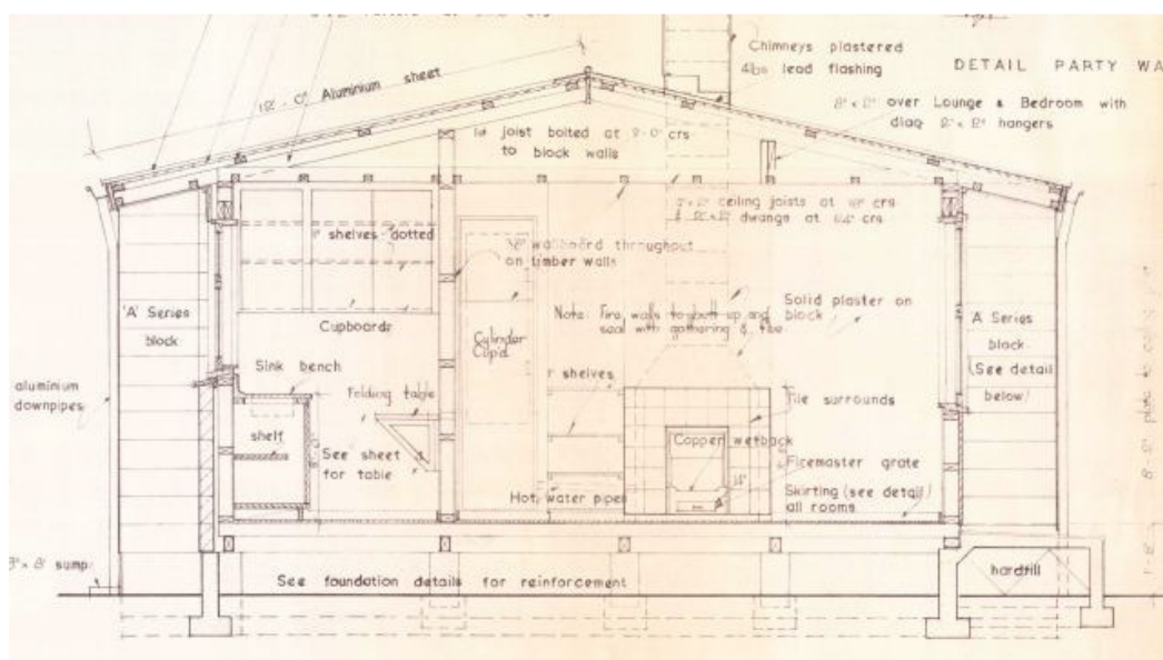
Figure 5: Typical cross section (note chimneys have been removed).
